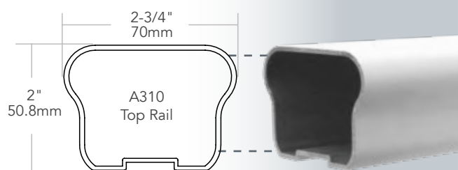
Top Rail
