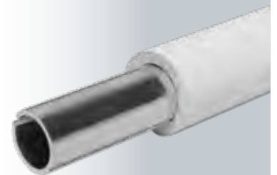
1-1/2" or 2" Vinyl Aluminum Reinforced ADA Handrailing Profile
