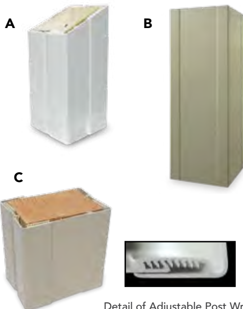
Detail of Adjustable Post Wrap Ratcheting System Adjustable in 0.125" Increments
