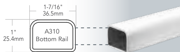
Bottom Rail
